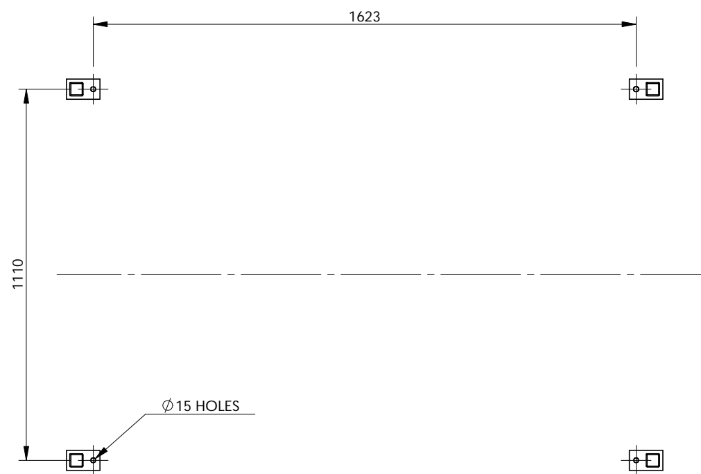
PLAN VIEW 1 : 12 MOUNTING HOLE POSITIONS ONLY
